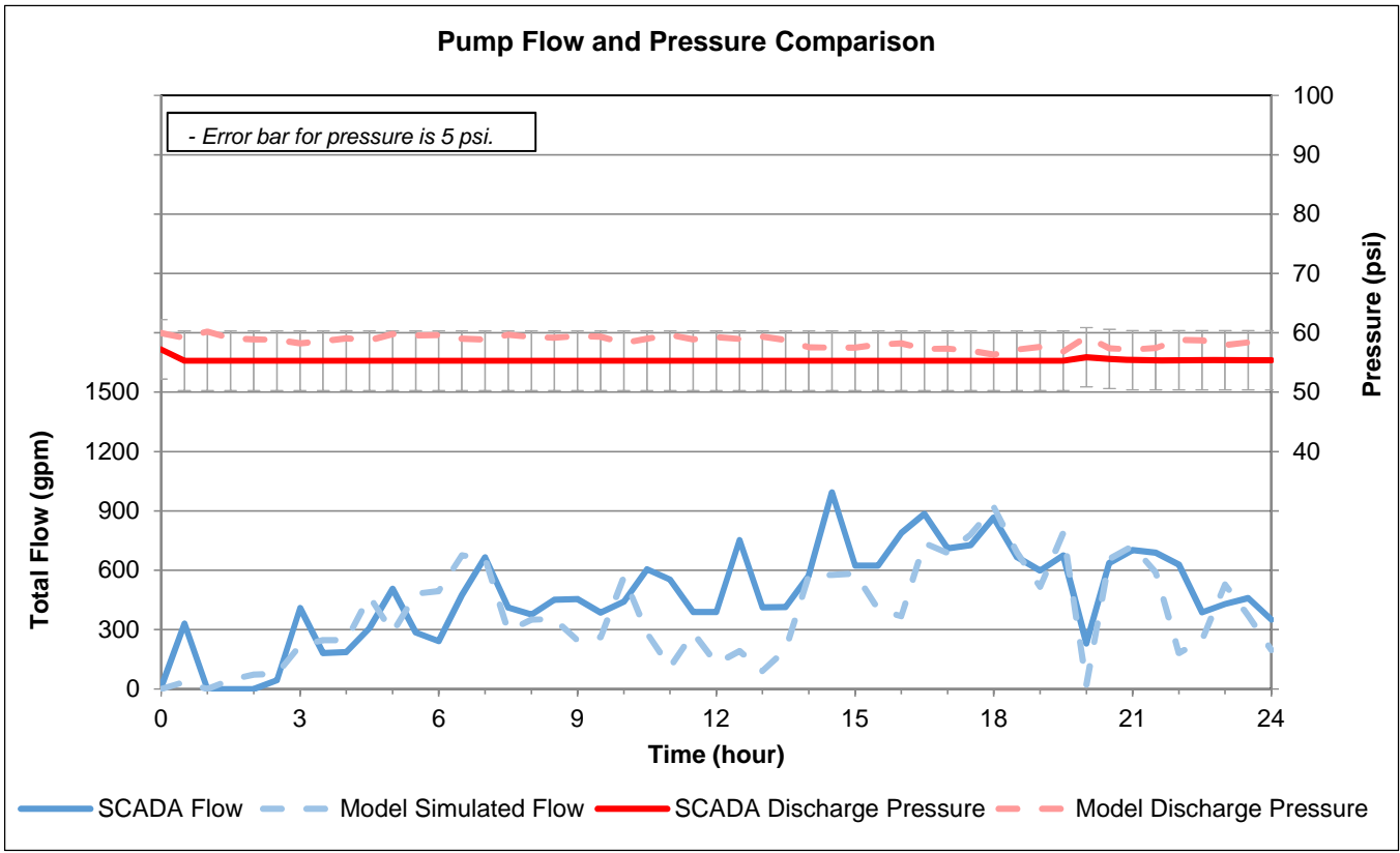
Figure 15. Tank 8 Comparison December 3, 2015
