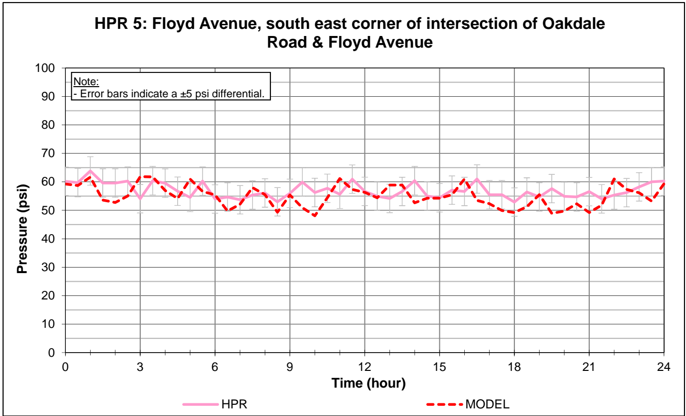
Figure 3. Round 1 HPR 5 and 8 December 3, 2015
