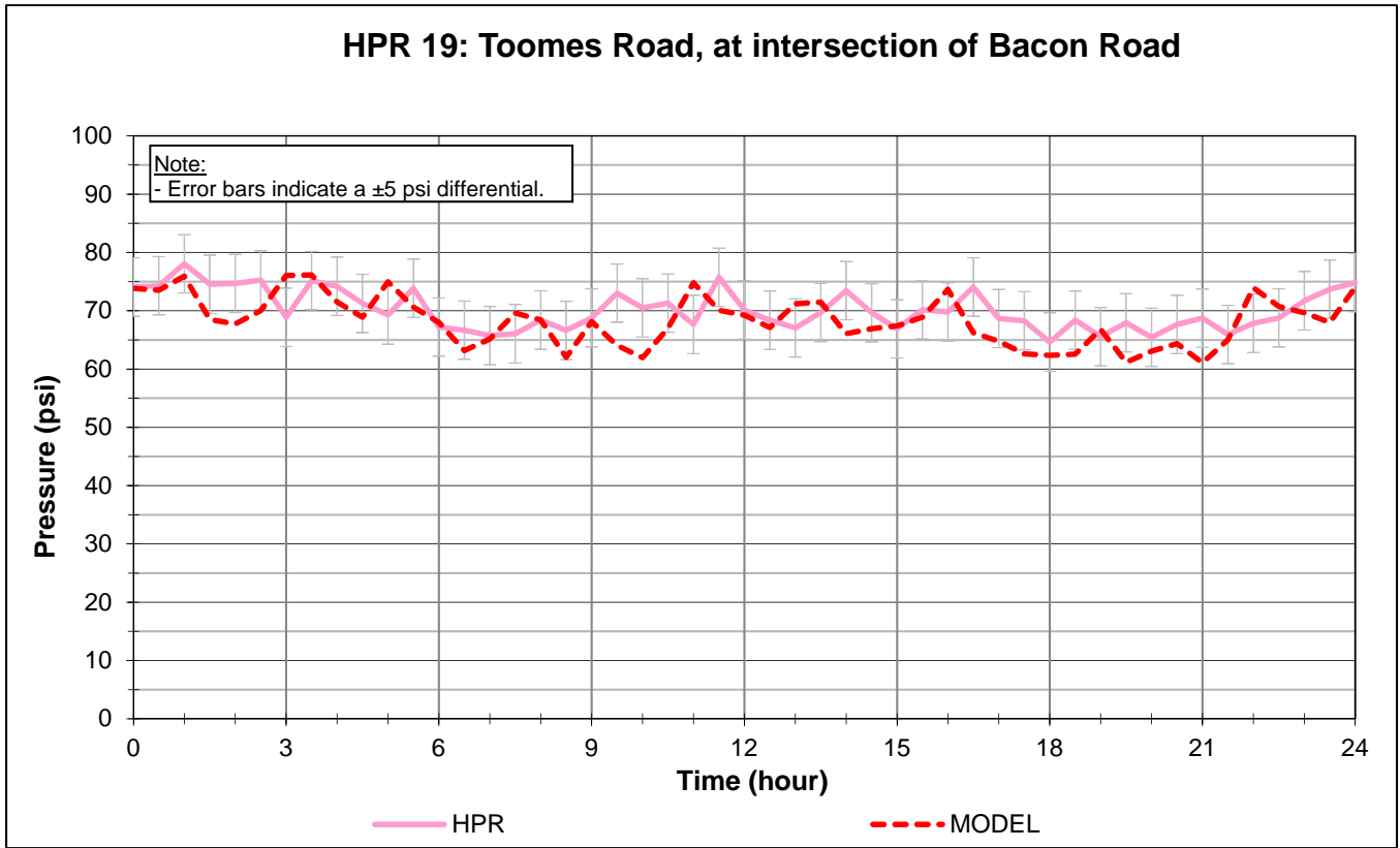
Figure 8. Round 1 HPR 19 and 20 December 3, 2015
