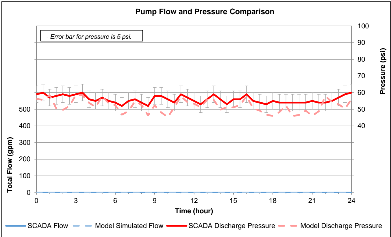
Figure 9. MID Tank Comparison December 3, 2015
