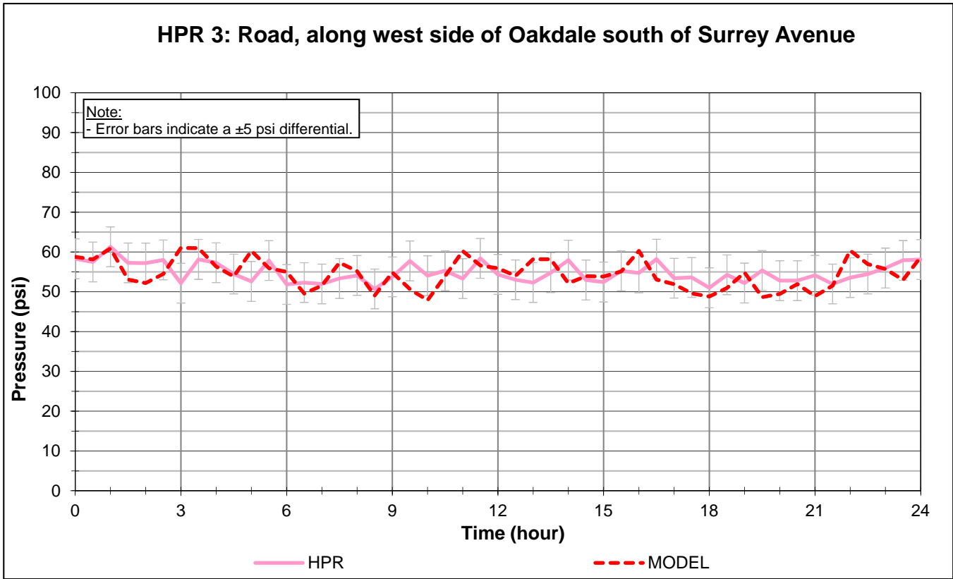
Figure 2. Round 1 HPR 3 and 4 December 3, 2015
