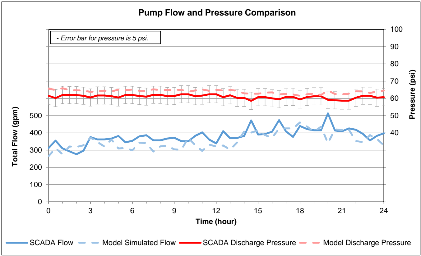
Figure 16. Tank 10 Comparison December 3, 2015
