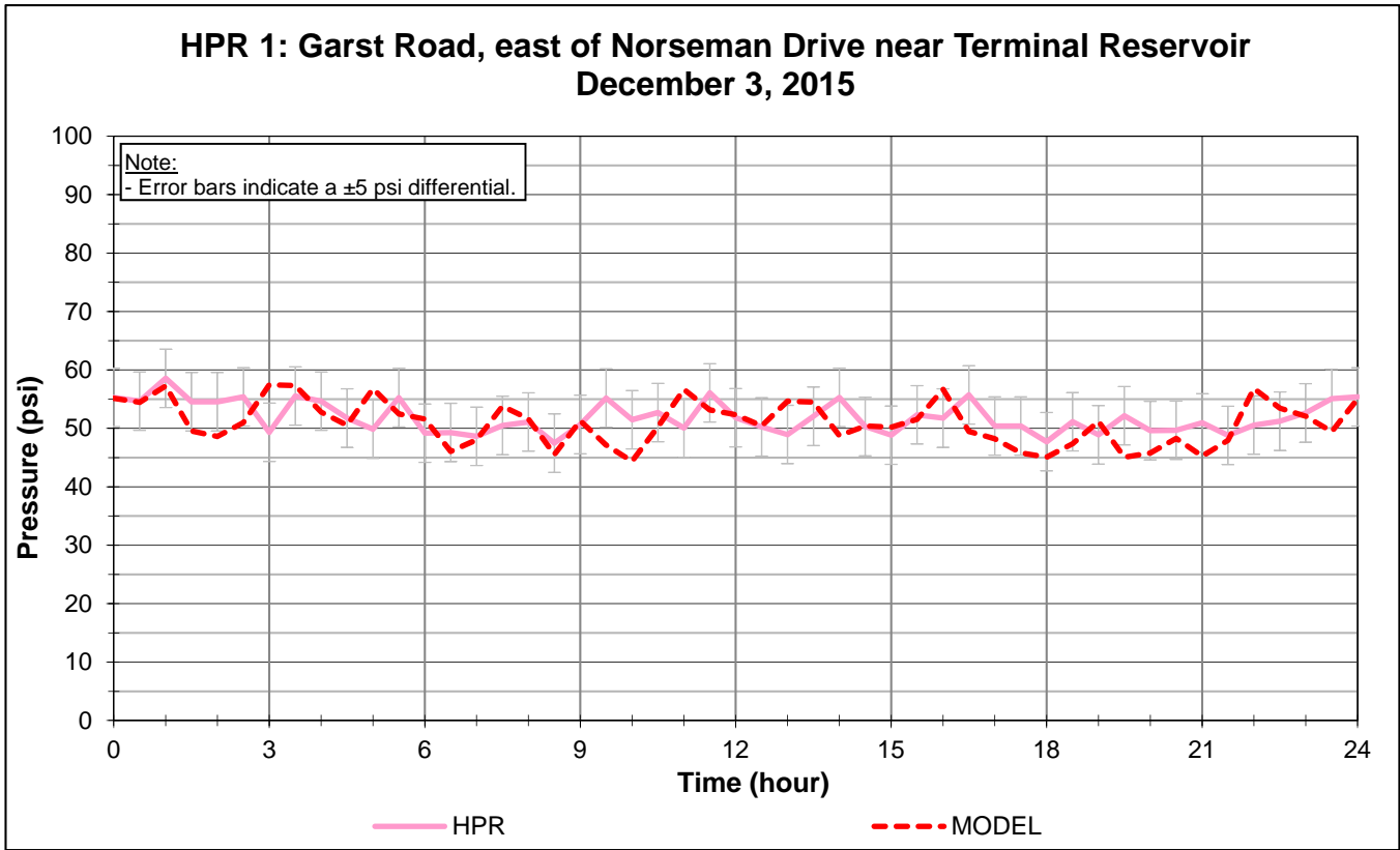
Figure 1. Round 1 HPR 1 and 2 December 3, 2015
