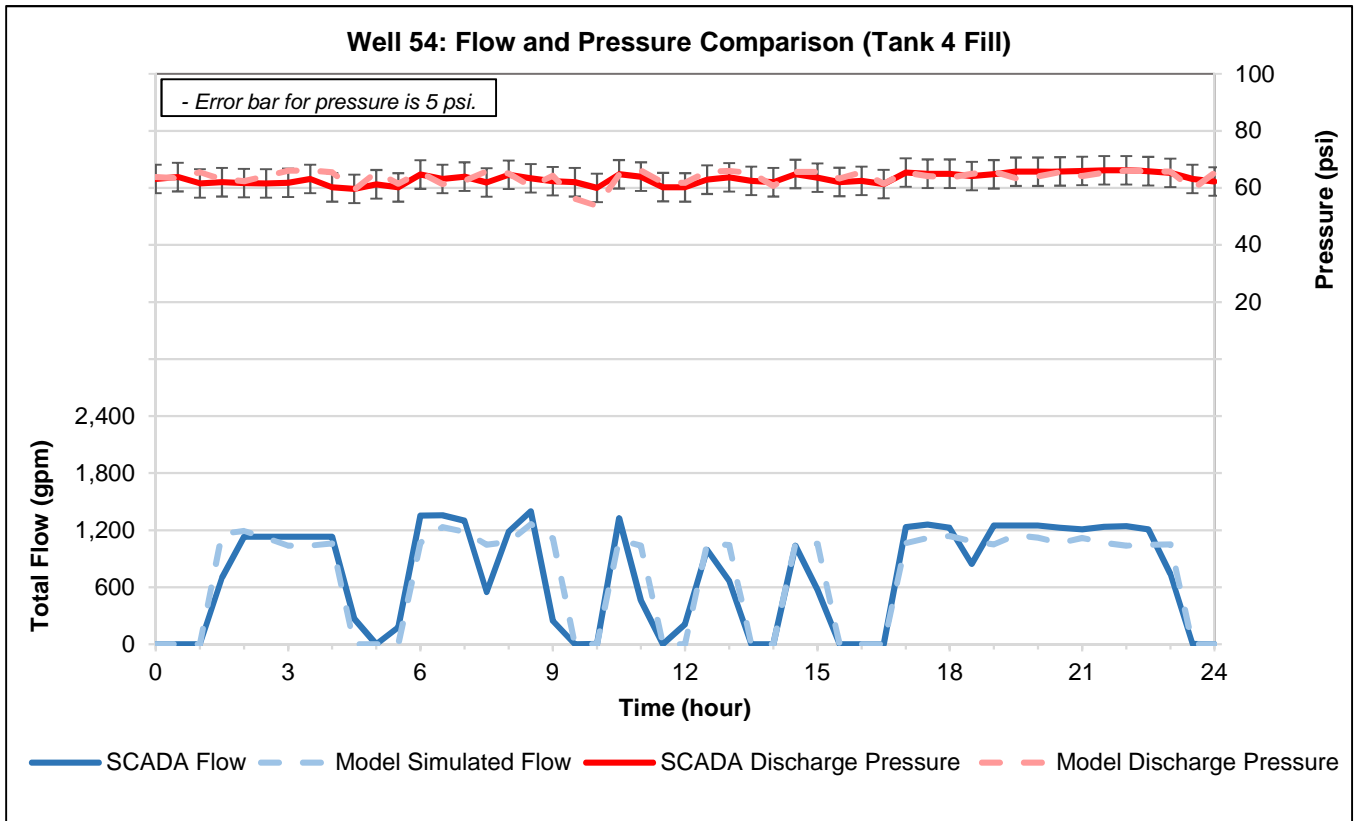
Figure 20. Well 54 and 58 December 3, 2015
