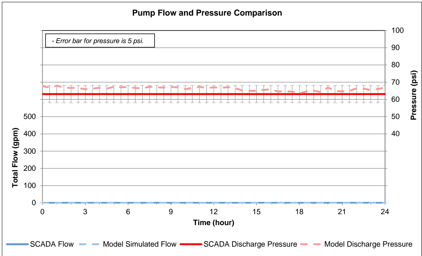
Figure 10. Tank 3 Comparison December 3, 2015
