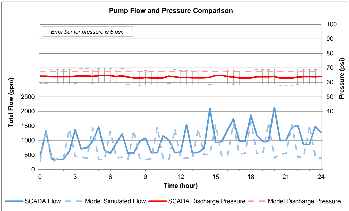
Figure 13. Tank 6 Comparison December 3, 2015
