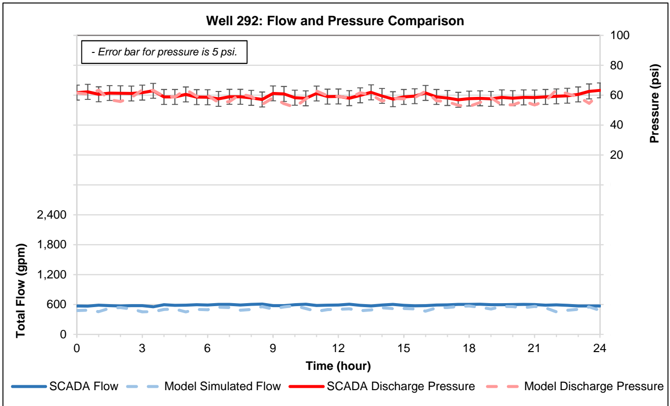
Figure 26. Well 292 and 297 December 3, 2015
