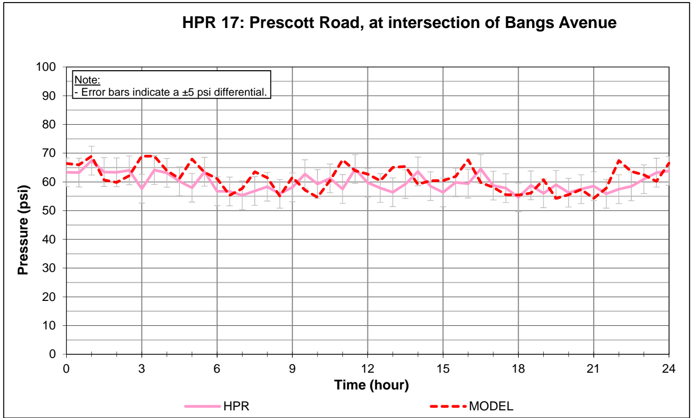
Figure 7. Round 1 HPR 17 and 18 December 3, 2015
