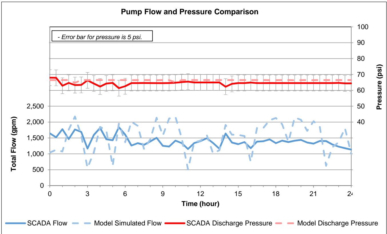
Figure 12. Tank 5 Comparison December 3, 2015
