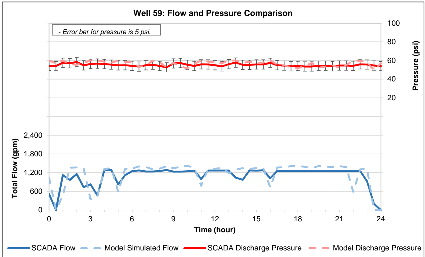
Figure 21. Well 59 and 62 December 3, 2015
