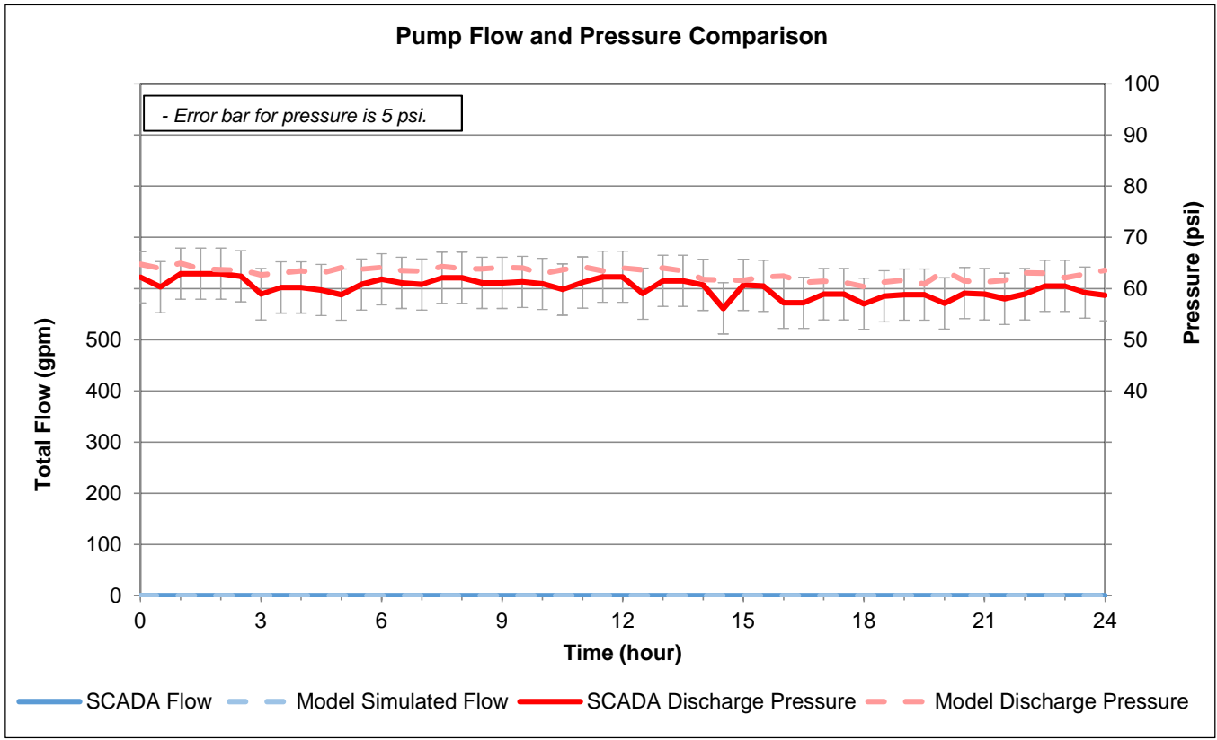
Figure 14. Tank 7 Comparison December 3, 2015
