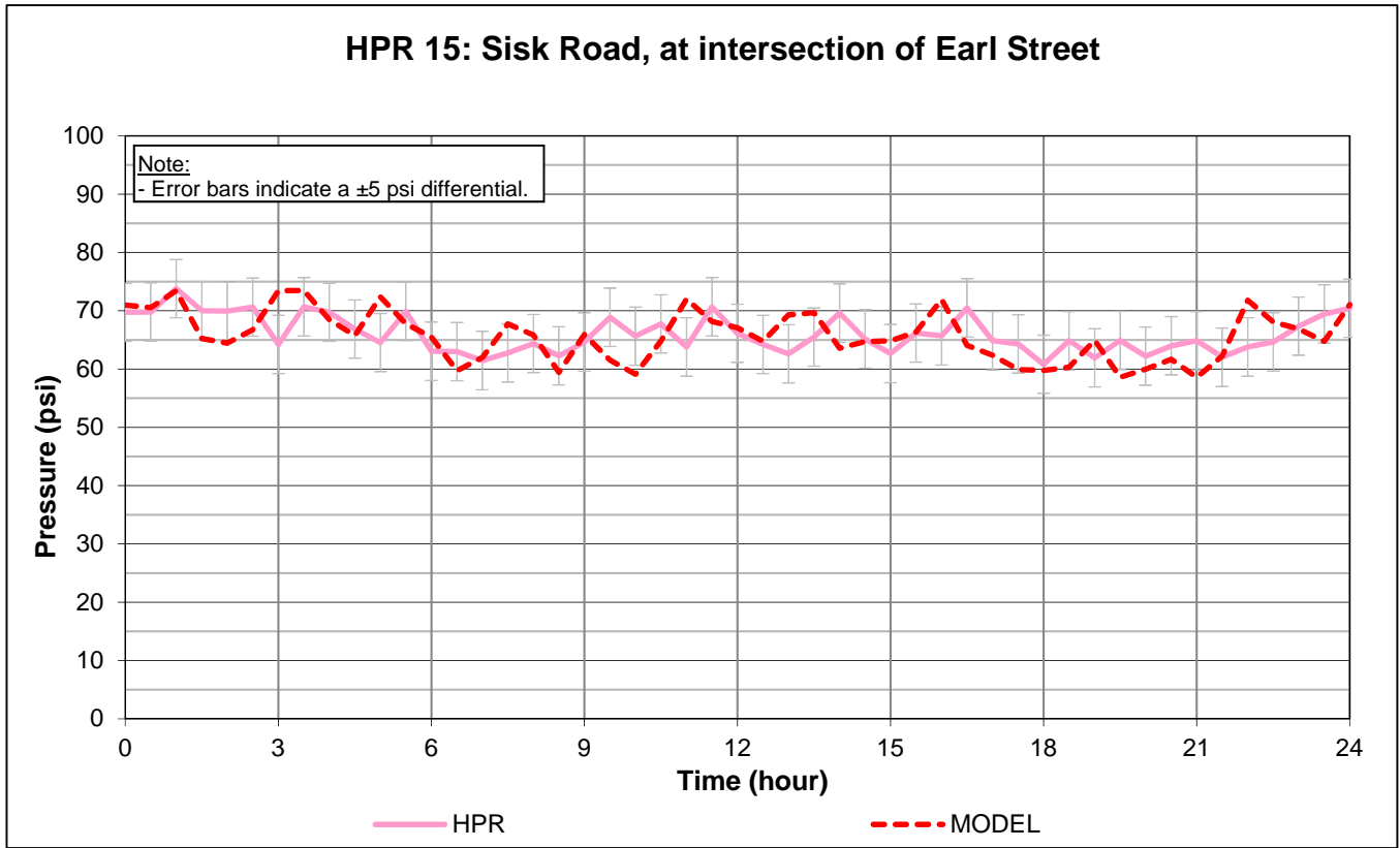
Figure 6. Round 1 HPR 15 and 16 December 3, 2015
