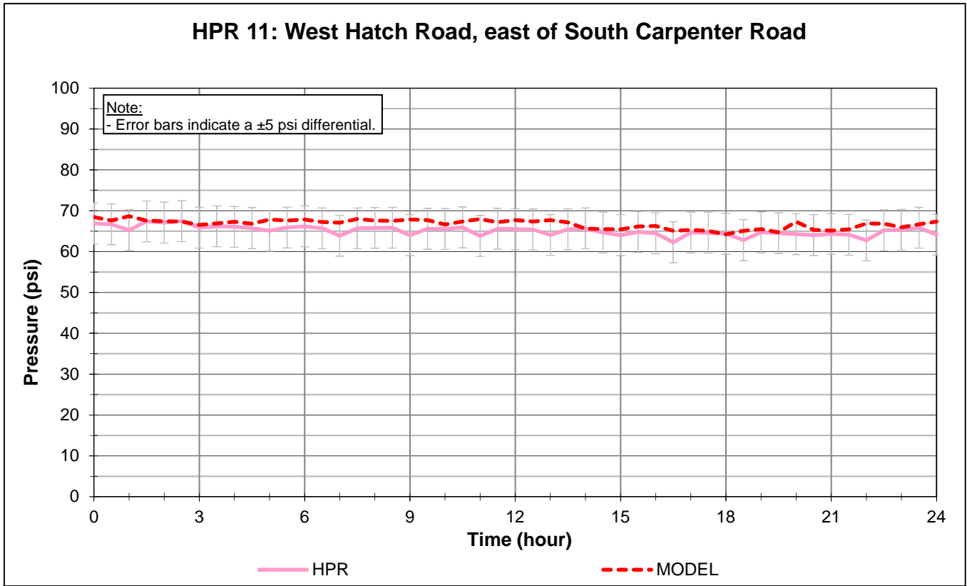
Figure 4. Round 1 HPR 11 and 12 December 3, 2015
