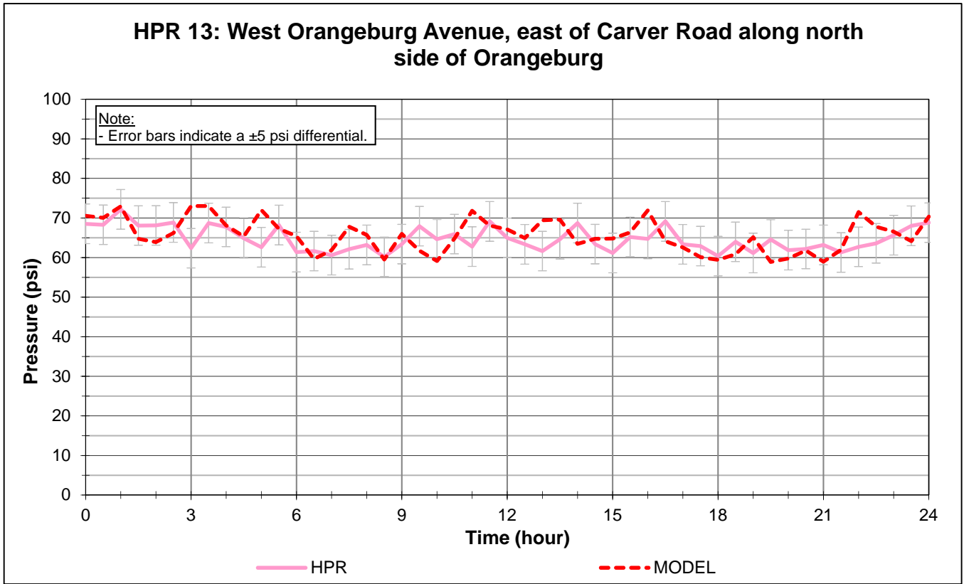
Figure 5. Round 1 HPR 13 and 14 December 3, 2015
