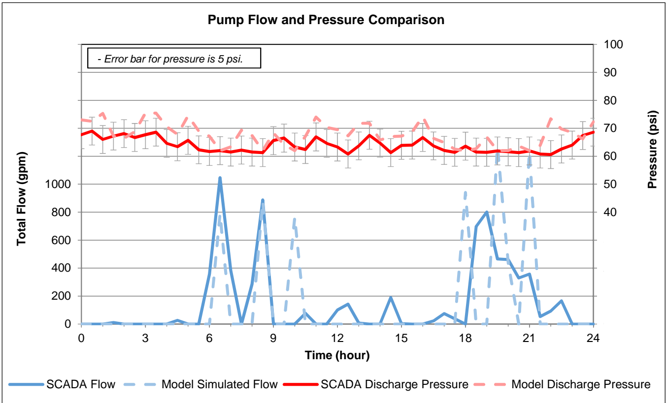
Figure 17. Tank 12 Comparison December 3, 2015
